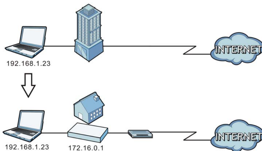
Figure 143 IPnP Application
