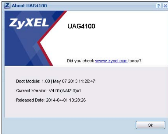
Figure 4 About
