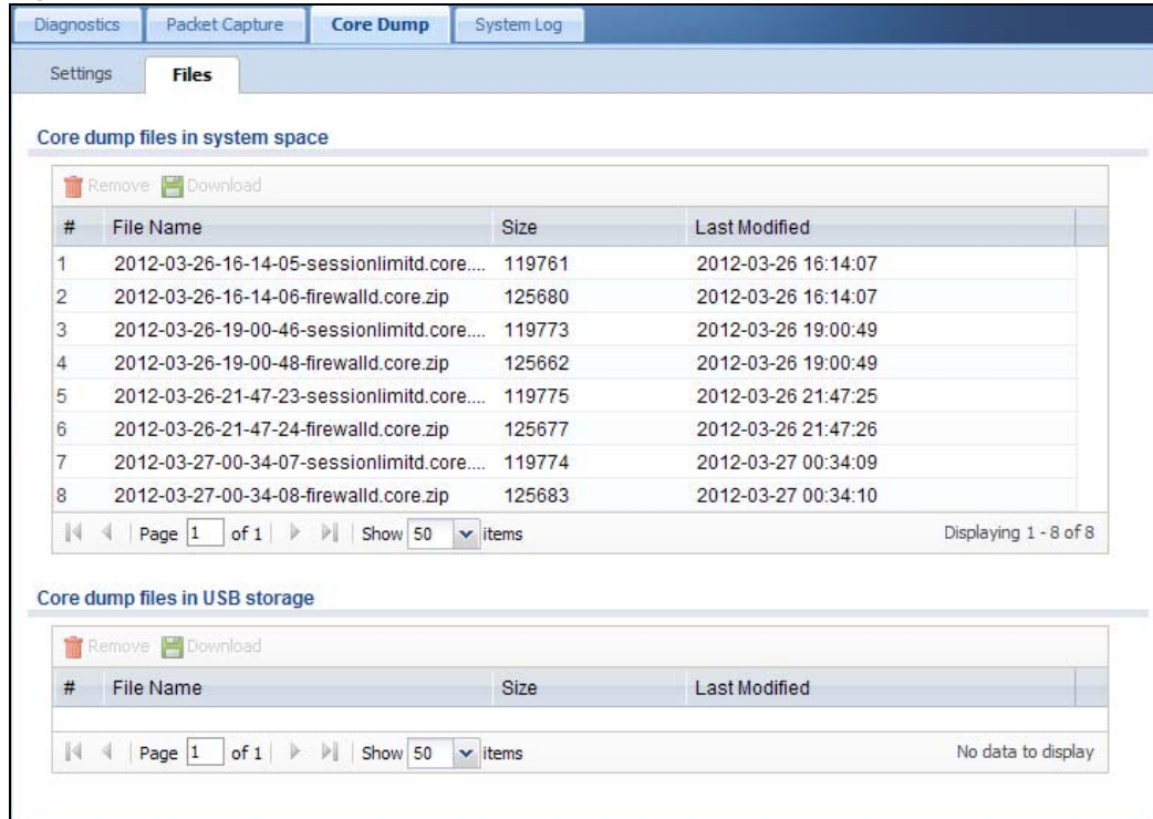
Figure 306 Maintenance > Diagnostics > Core Dump > Files
