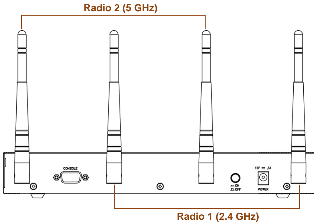
Figure 18 Rear Panel
