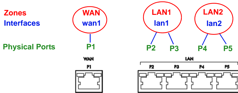
Figure 1 Zones, Interfaces, and Physical Ethernet Ports
