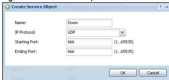
Figure 171 Firewall Example: Create a Service Object
