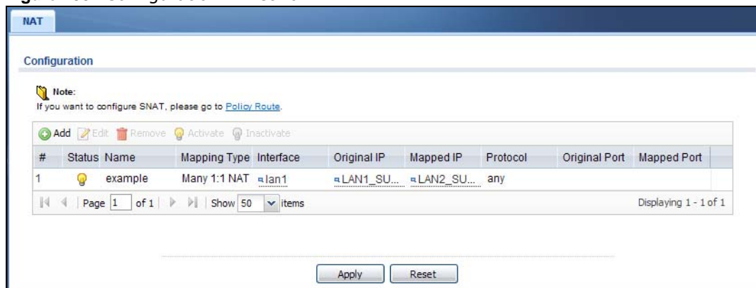
Figure 108 Configuration > Network > NAT
