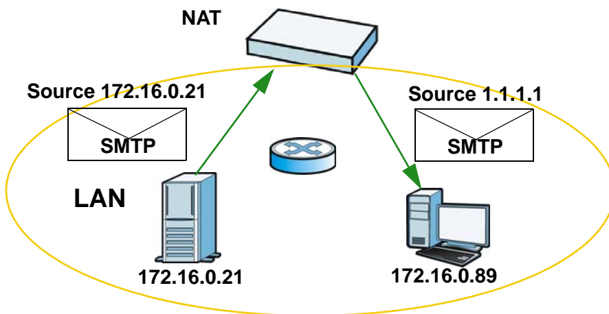
Figure 112 LAN to LAN Return Traffic
